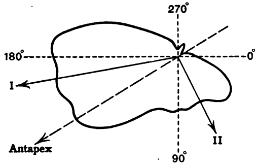
VIII. Region XIII. ; centre R.A. 13^{\text{h}} 12^{\text{m}} , Dec. +17^{\circ} .
